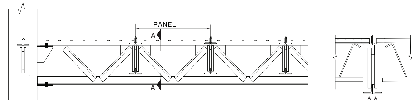
TRUSS SUPPORTED BY COLUMN [MOMENT CONNECTION] JOISTS ARE ONLY SUPPORTED BY THE TRUSS
