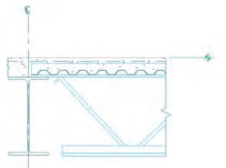
Figure 17. Typical Vescom Joist to Wide-flange Beam Connection
