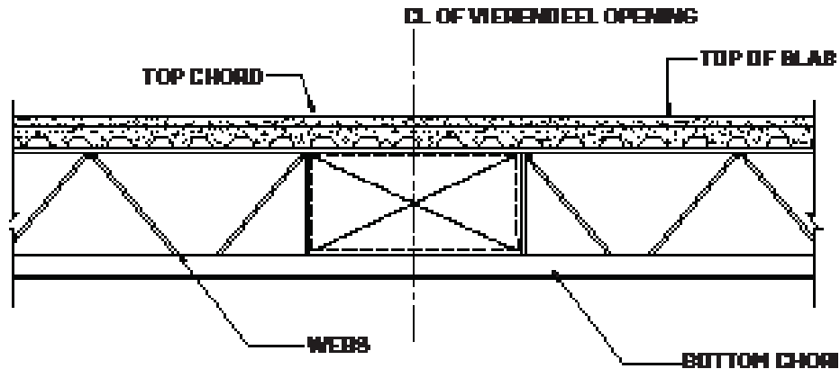
Figure 9. Typical Vescom Joist Vierendeel Opening
